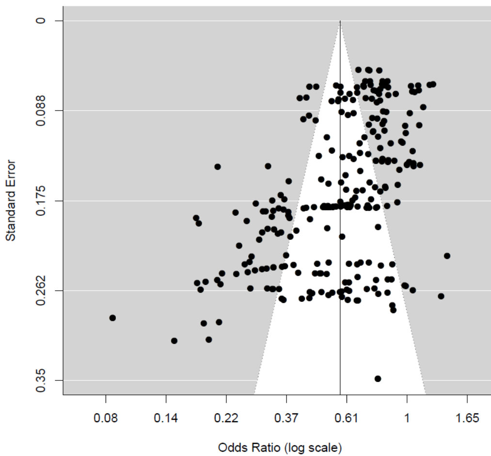
Figure 1.3: Funnel plot
